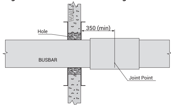
Figure 7 - Standard Wall Crossing
