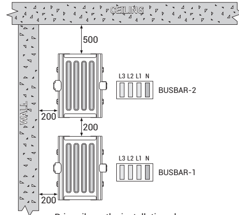
Figure 2 - Edgewise Application
