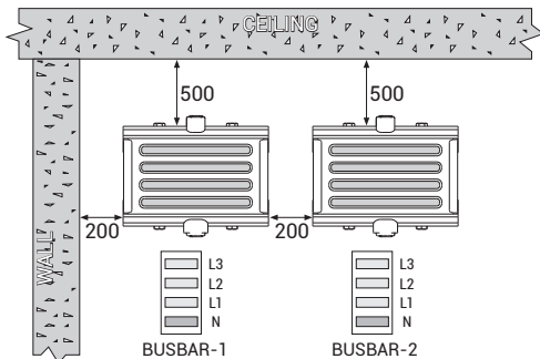
Figure 3 - Flatwise Application
